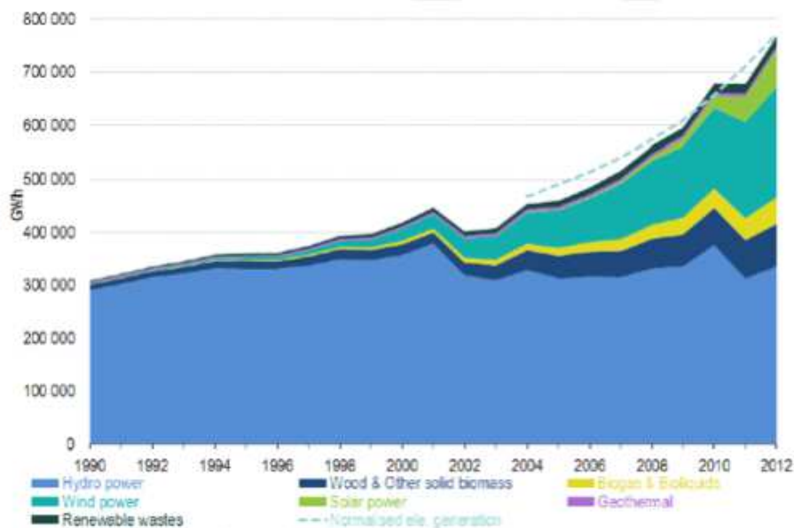
The gross electricity generation from renewable energy sources in the EU-28
