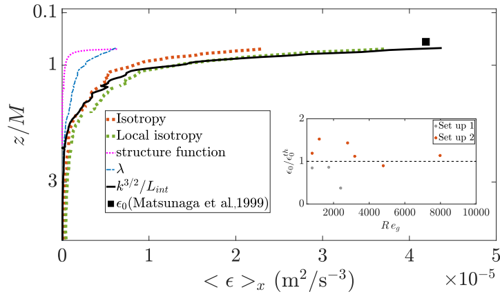
FIGURE 4.8 – Vertical profiles of the dissipation rate calculated from five definitions with different assumptions. Inset plot : comparison of \epsilon_0 obtained experimentally with its theoretical expression in eq. (4.4) (Matsunaga et al. , 1999).
