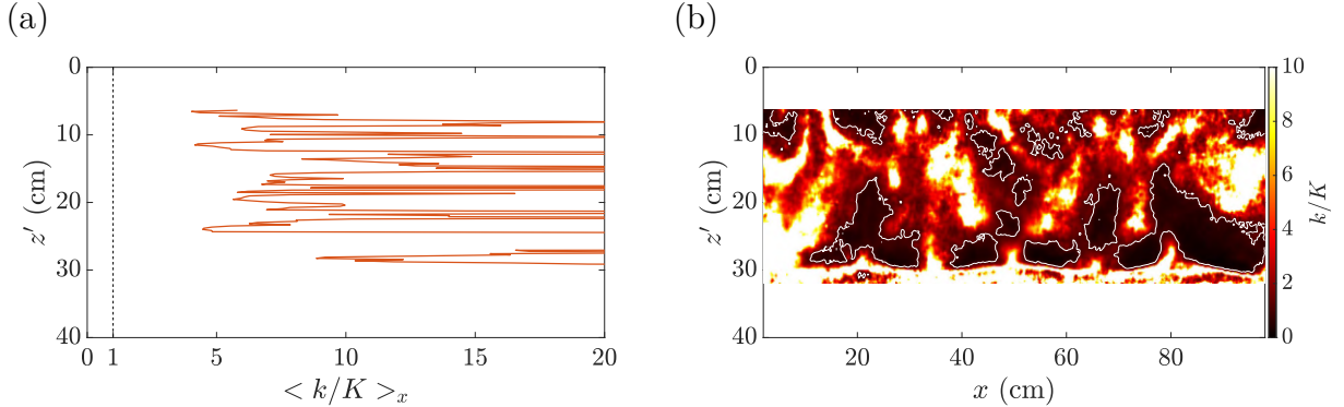
FIGURE 4.12 – Example at Re_g = 800 and at time t_6 of : (a) Depth profile of the turbulent kinetic energy, k , over the kinetic energy based on the mean flow, K . (b) Map of k/K to ensure that the turbulence is homogeneous. The white contour line represents k = K .
